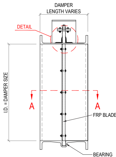
SECTION B
