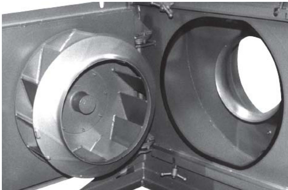
Heavy duty ball bearings provide door support.
